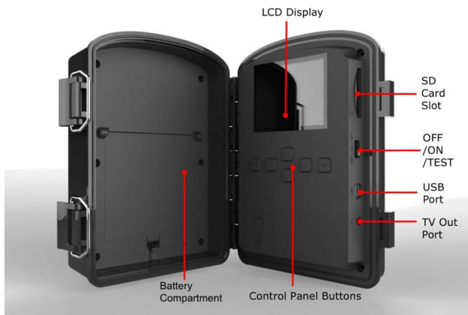
Interior View
