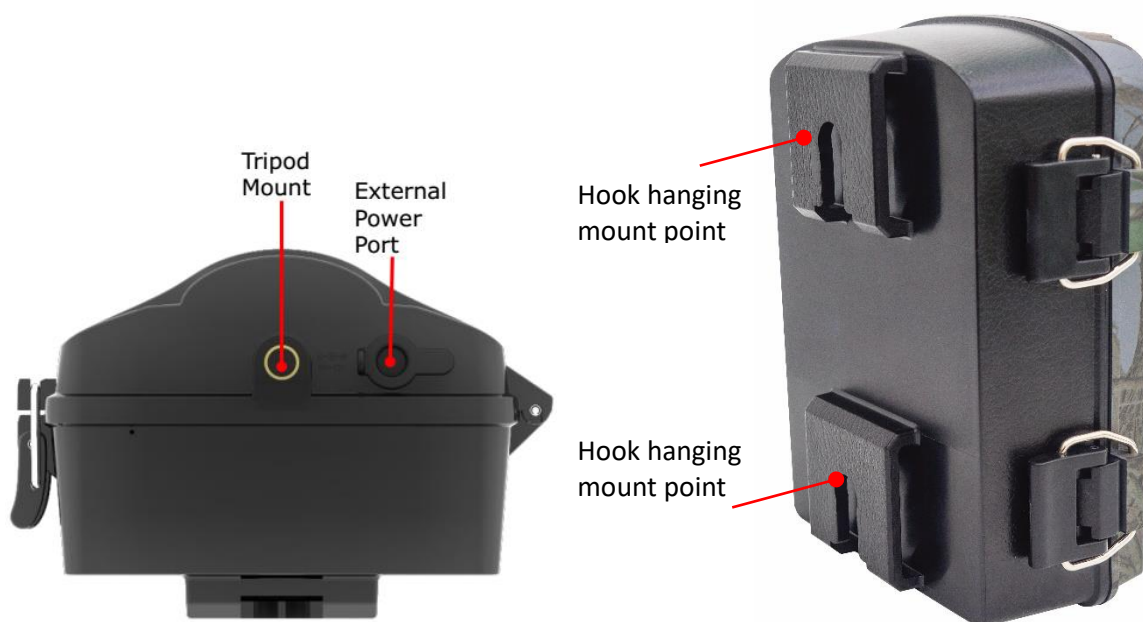
Bottom View
